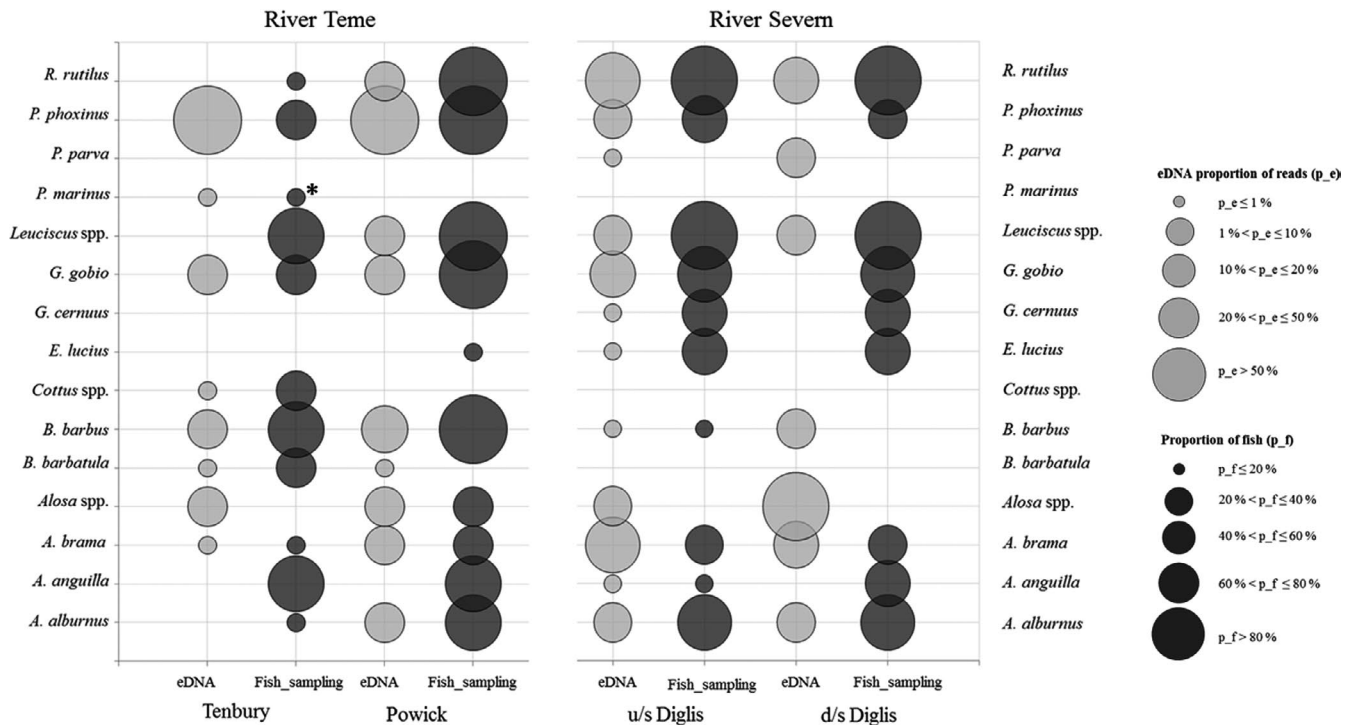
FIGURE 2 Bubble graph showing the relative abundance of 15 fish species detected by eDNA metabarcoding and fish survey above and below the main impoundment on both rivers. For eDNA, this was based on proportion of the number of reads (after bioinformatics filtering and minimum threshold reads applied); for fish surveys, it was the proportion of individuals caught through fish surveys (total number of species detectable through eDNA metabarcoding). * Lamprey detected at Tenbury without a clear species assignment
